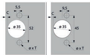
Bohrbild HETTICH TH 53 ø 10x11 THS55 ø 10x6
