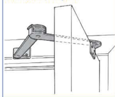
Fix 328A on opening side
