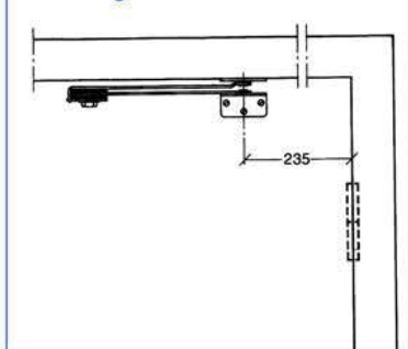
Mounting instructions Fix 328
