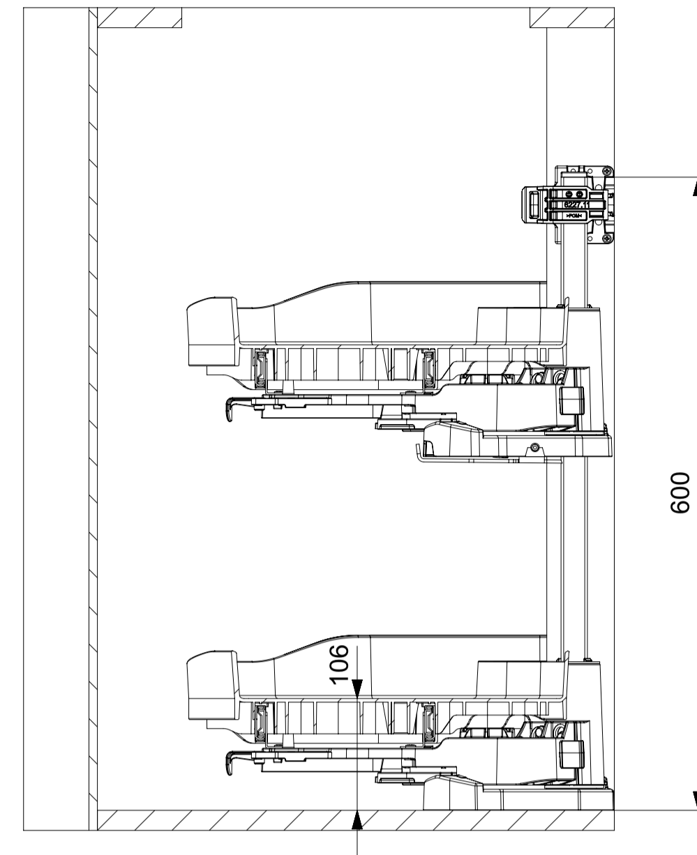
SECTION F-F
